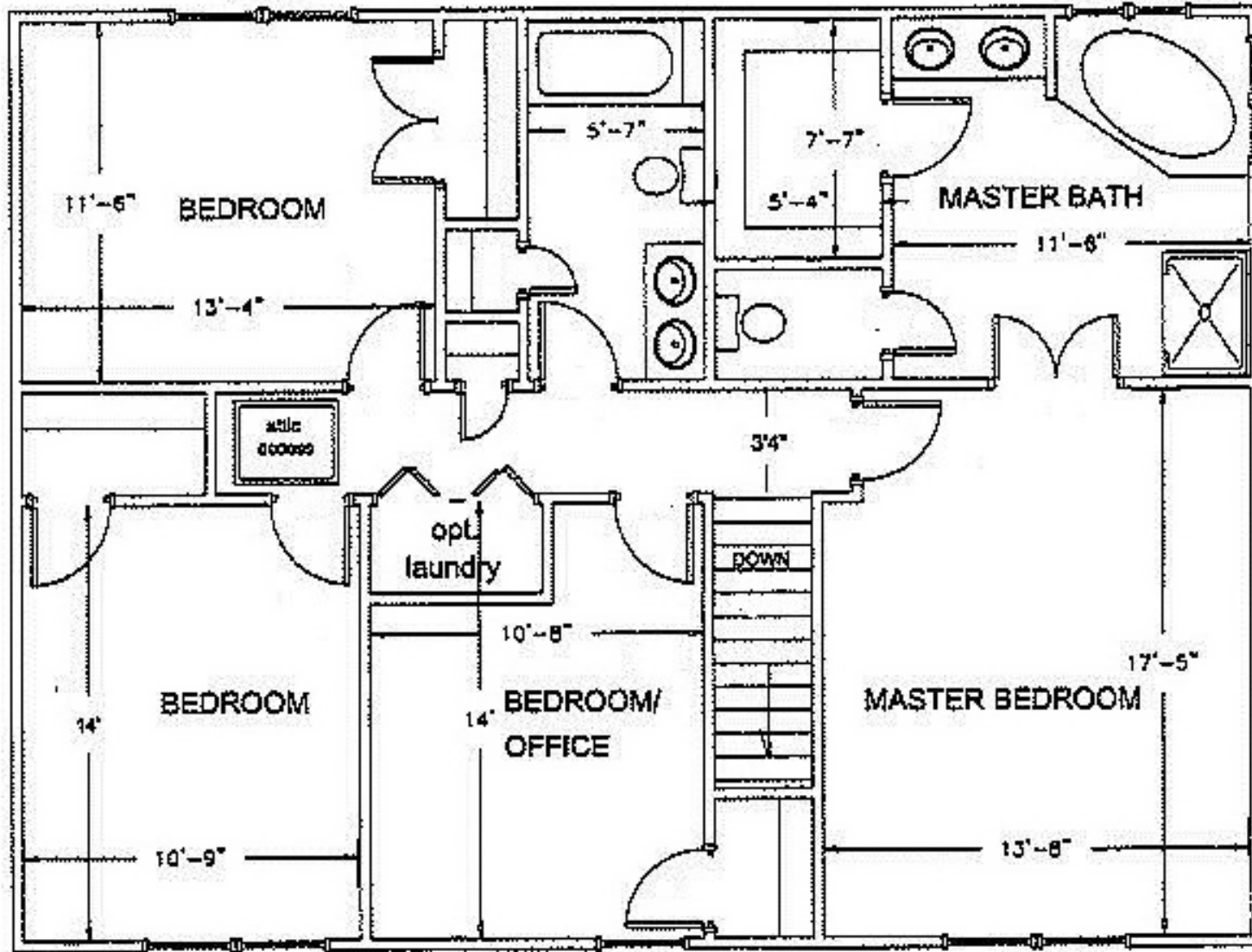
2nd Floor
