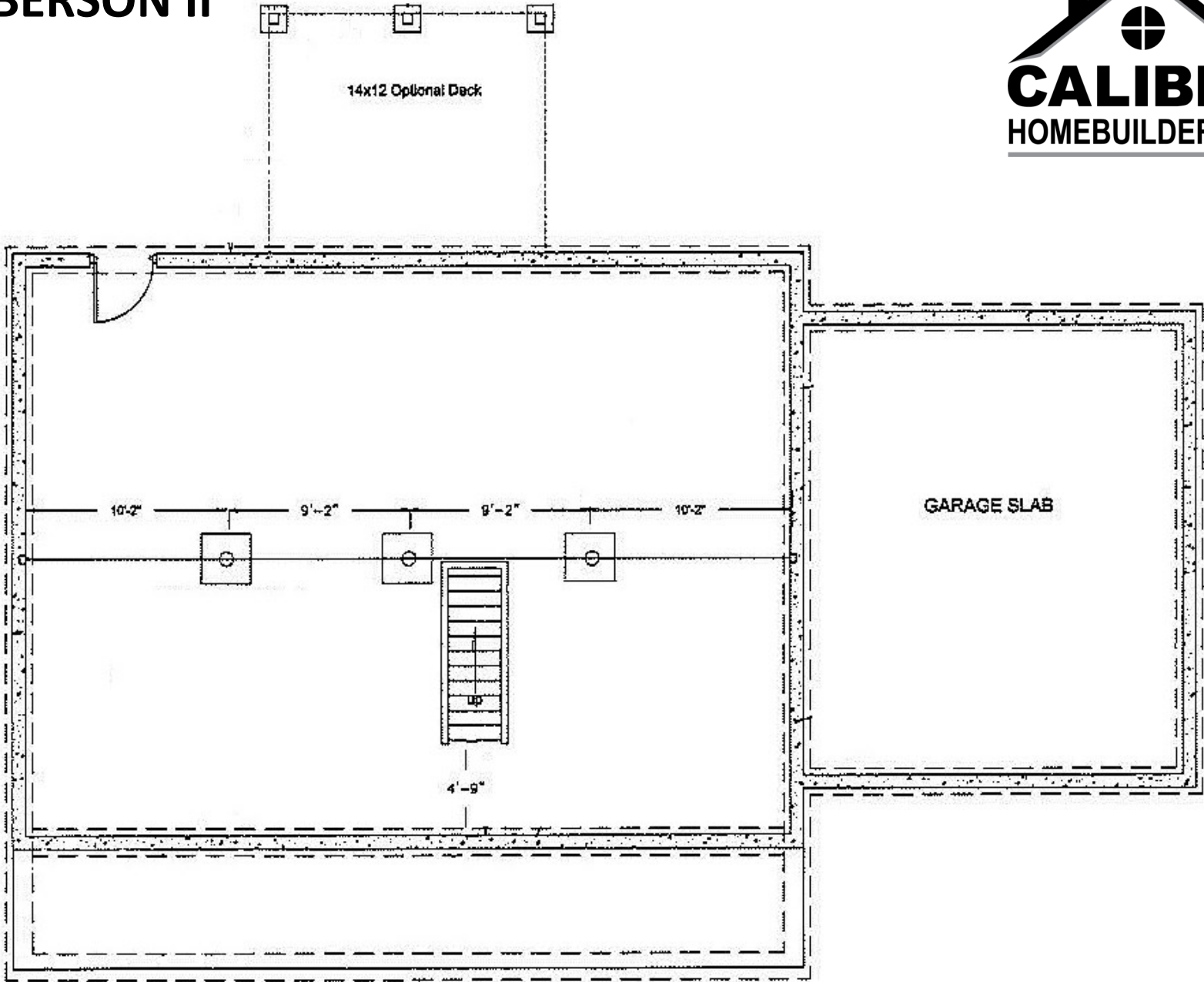
Basement
